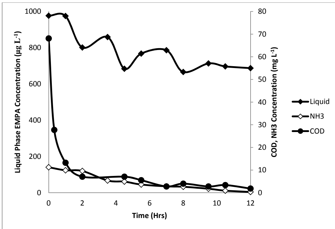
Figure 5: EMPA Biodegradation: 1 \text{mg L}^{-1} activated sludge at 25° C with nitrifiers active
